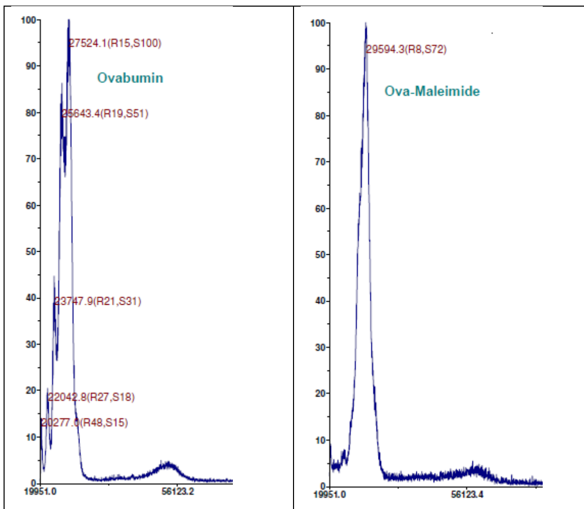
Figure 1: MALDI-TOF MS analysis of Ova (left) and purified conjugates (right) (M/2)
